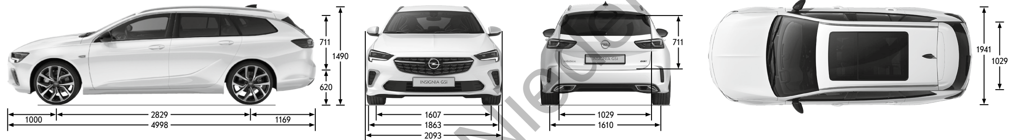
Sports Tourer Alle Maße in mm
