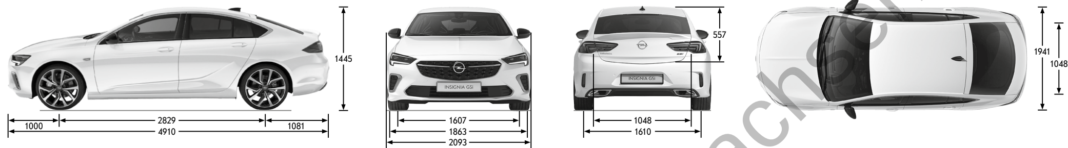
Grand Sport Alle Maße in mm
