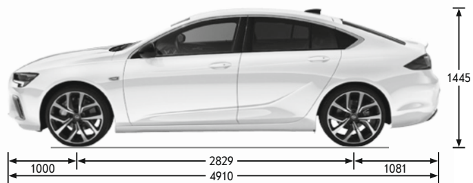
Grand Sport Alle Maße in mm
