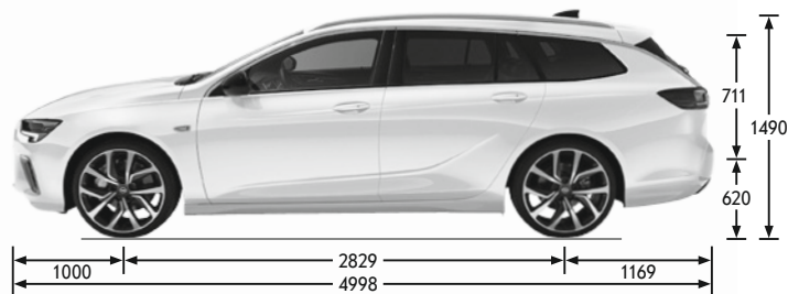
Sports Tourer Alle Maße in mm
